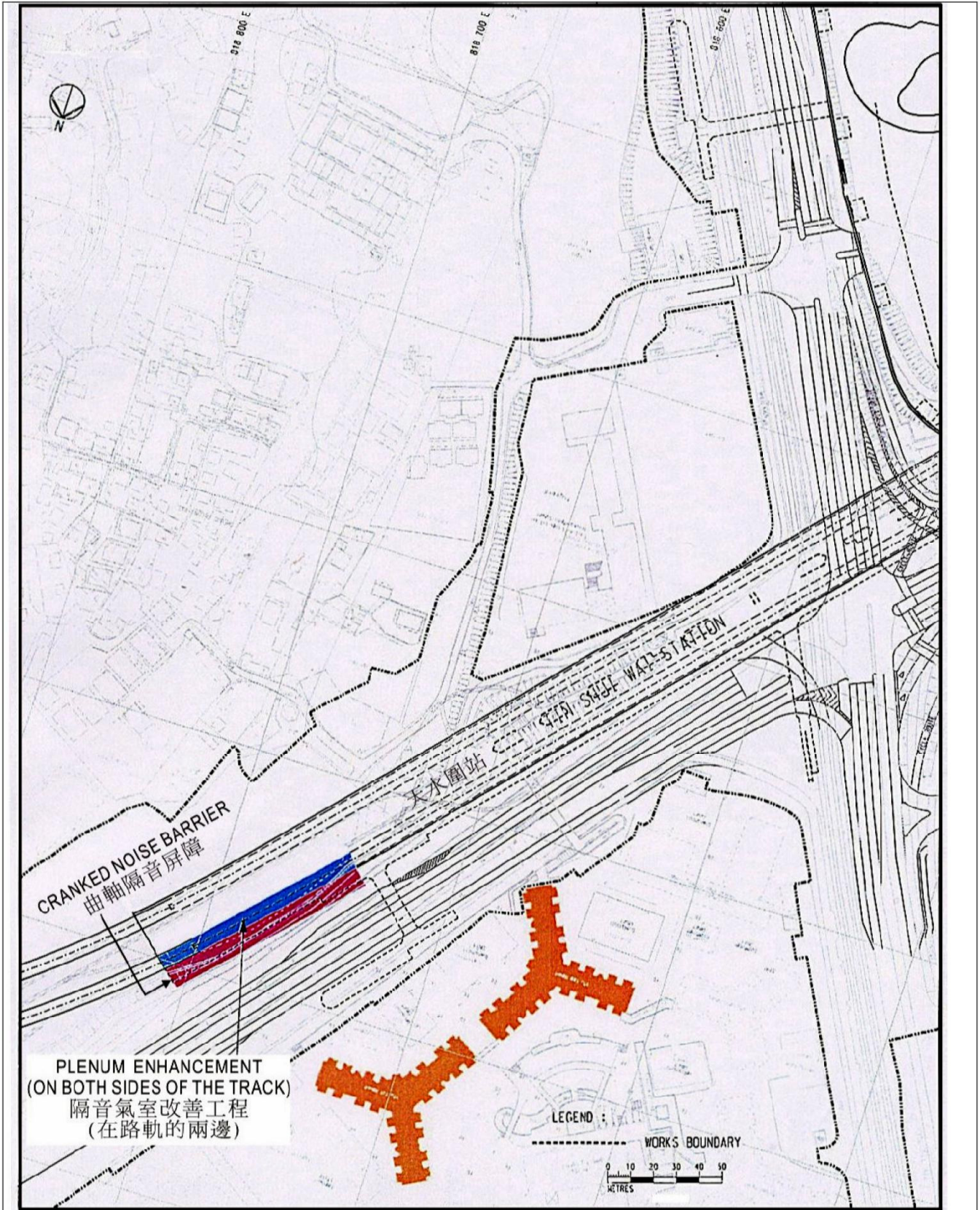
Figure 9 – Cranked Noise Barrier and Plenum Enhancement at the Tin Shui Wai Station 圖九 – 天水圍站的曲軸隔音屏障及隔音氣室的改善工程
